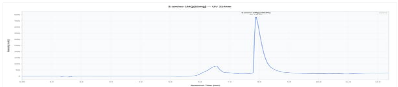
5-Amino-1MQ 50mg - PS07-5AM50: UV Chromatogram
